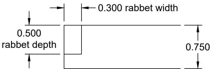
RABBET DETAIL
